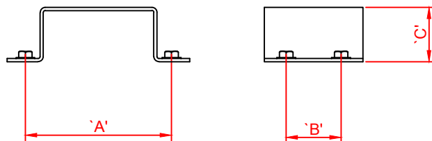
Mounting Bracket
