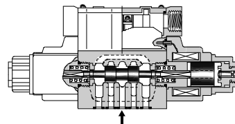
Plug-in Connector Type
