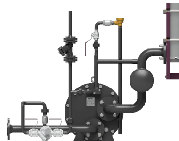
Optional pump trap set
