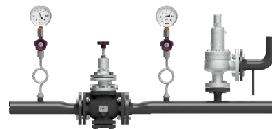
Optional pressure reducing set *
