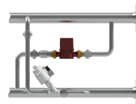
Optional pump & bypass set *
