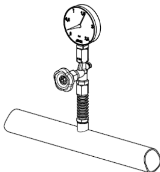
Horizontal pipe
