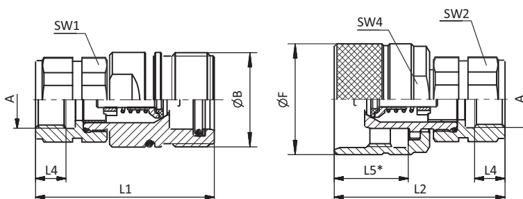
SW: Width across flats. All dimensions in mm * Insertion Female Body.
