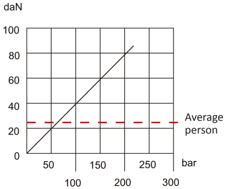
Effort (daN) operating on the end of the lever. Average person will generate 25 daN force.
