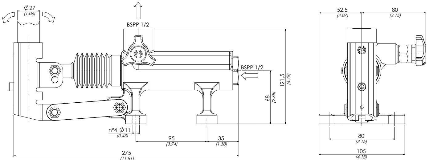
THE PUMP IS SUPPLIED WITH ACTING LEVER Length= 600mm
