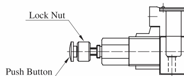
Plug-in Connector with Solenoid Indicator Light
