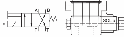
Reverse Mtg. of Solenoid
