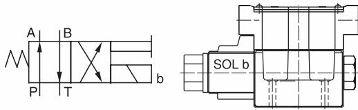
Standard Mtg. of Solenoid
