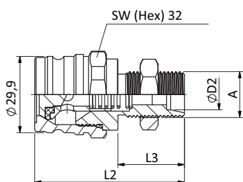
SW: Width across flats. All dimensions in mm
